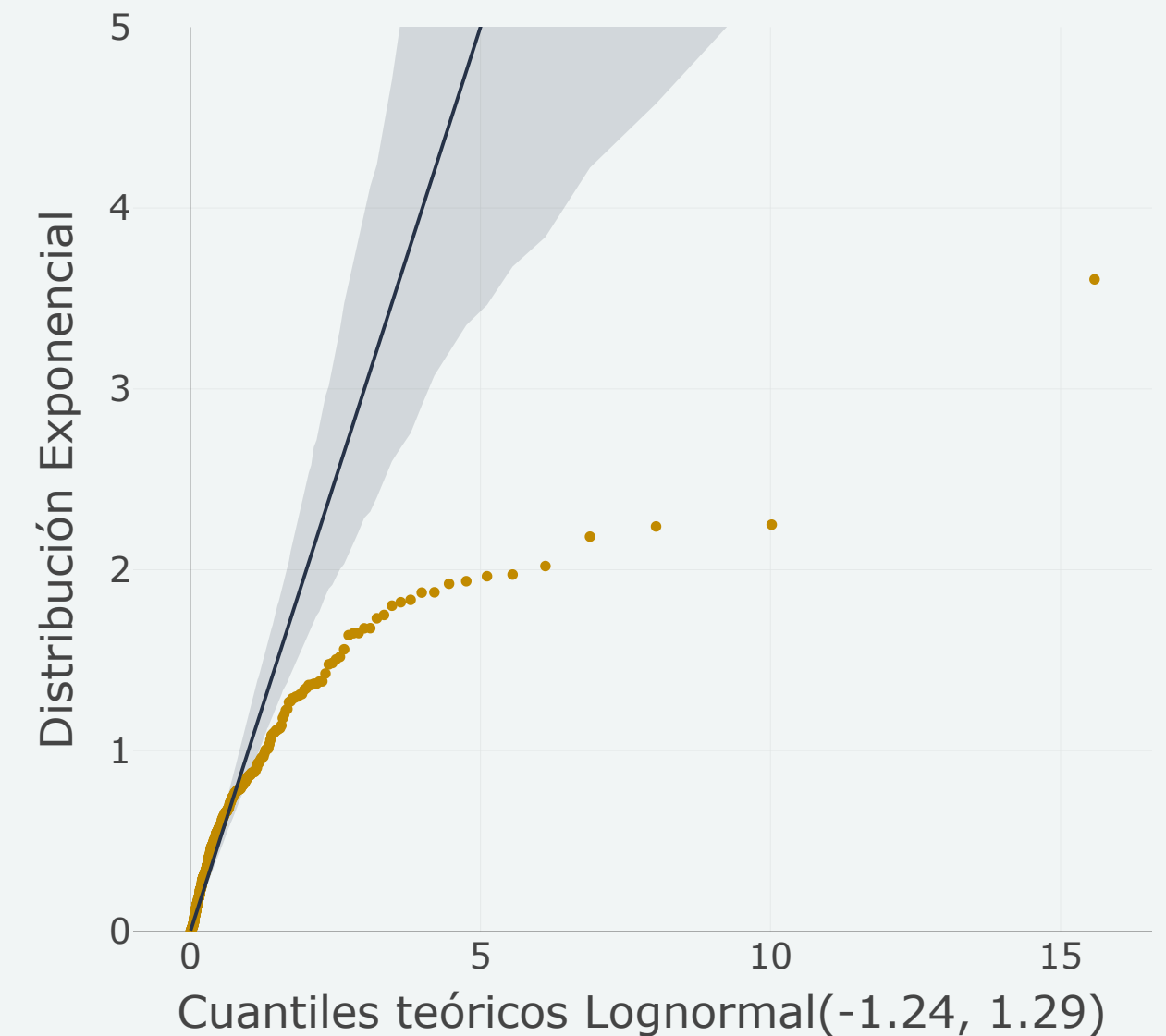
QQ-plot (lognormal)
