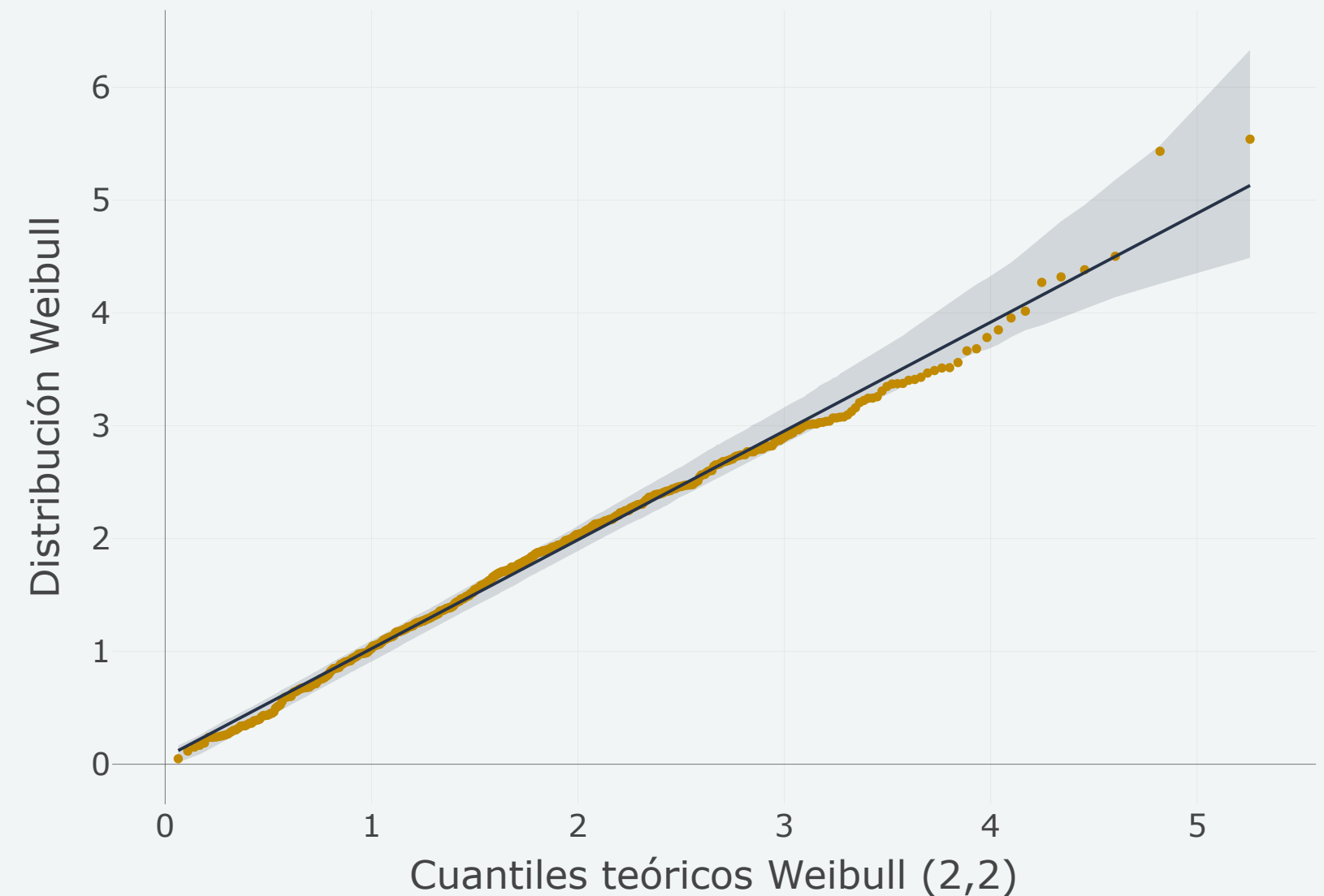
QQ-Plot (Weibull)
